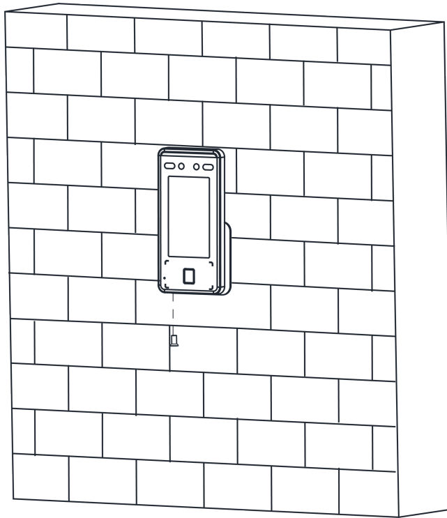
Figure 3-5 Secure Device
