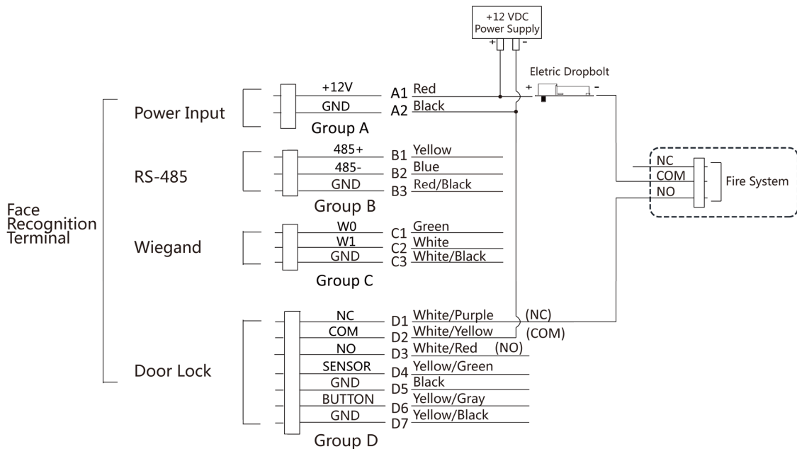
Figure 4-5 Wiring Device
