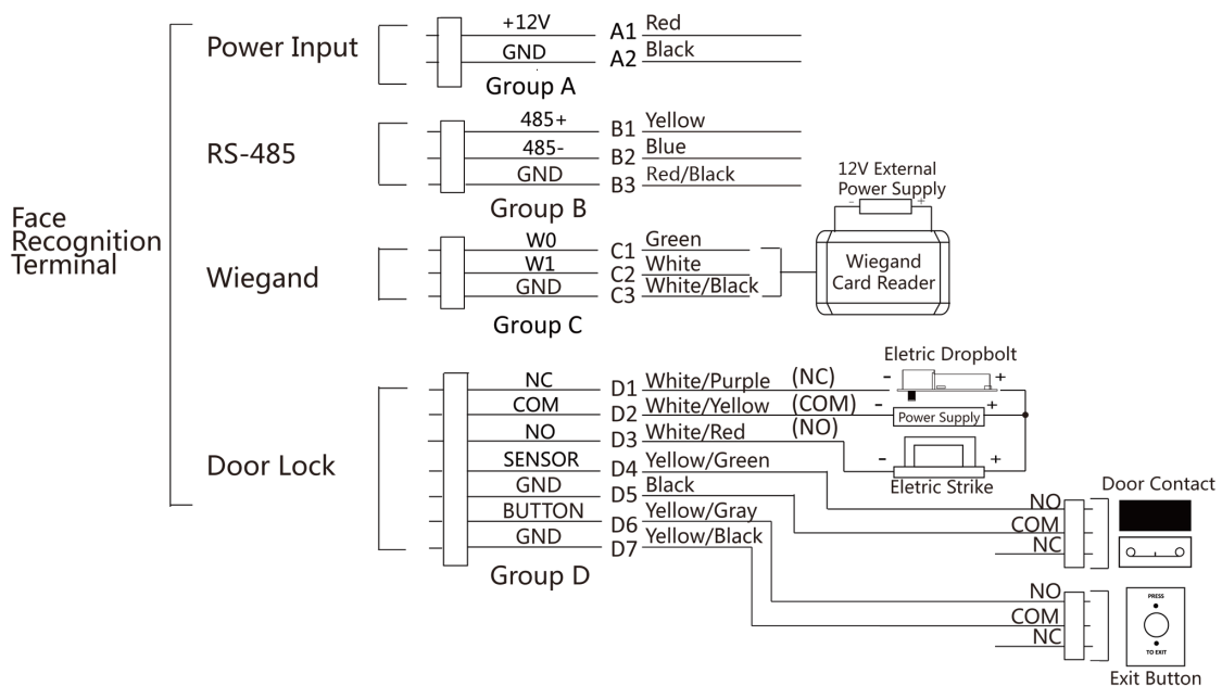
Figure 4-1 Device Wiring
