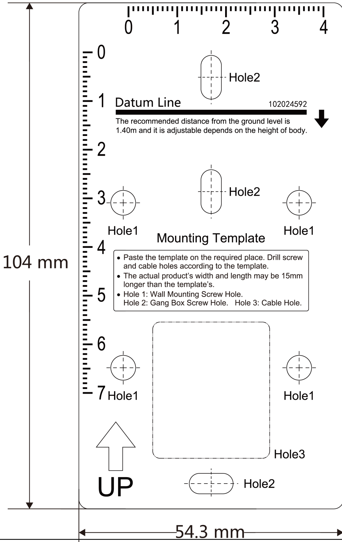
Figure 3-7 Mounting Template
