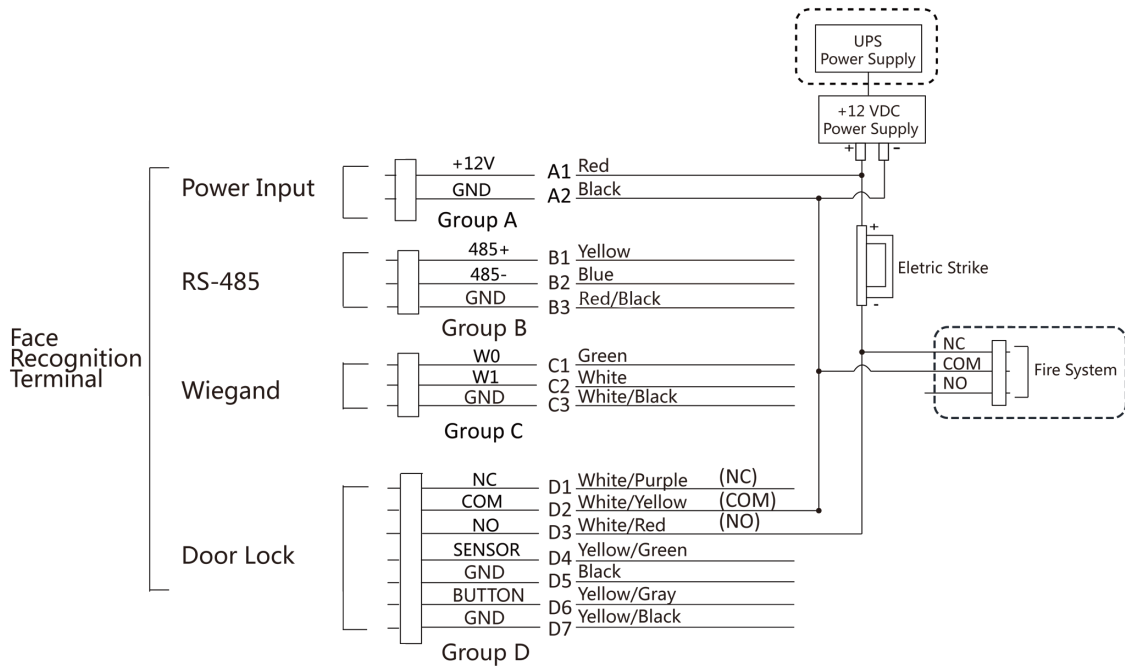
Figure 4-7 Device Wiring
