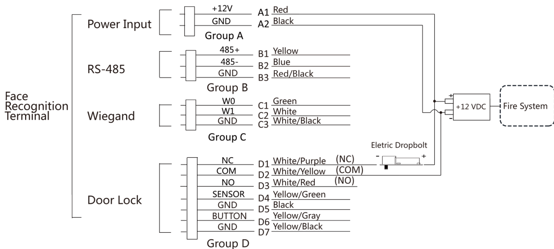
Figure 4-3 Wire Device
