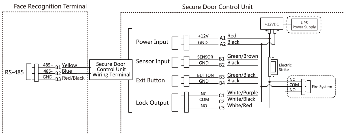
Figure 4-8 Wiring Diagram
